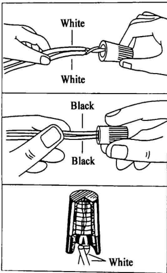
Figure 2-Wire Connectors
